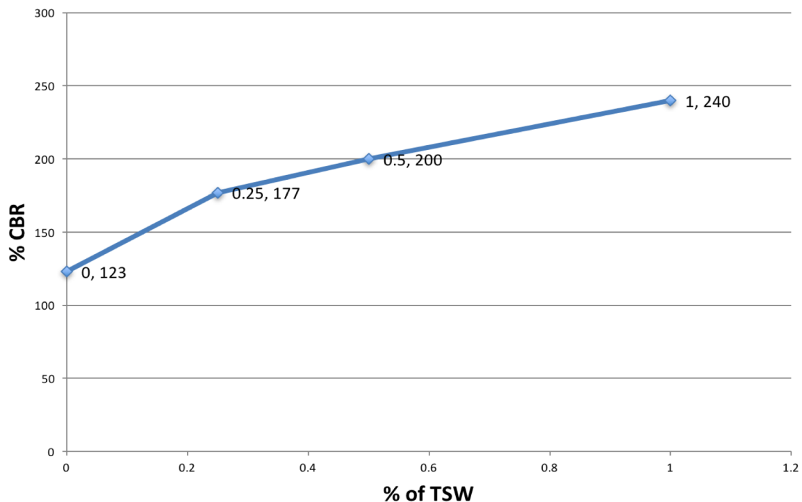
CBR Chart
