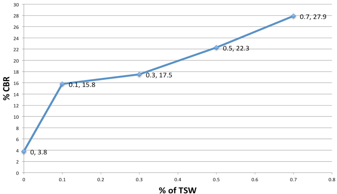
CBR Chart
